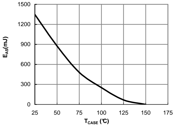
Figure 12: Avalanche energy
