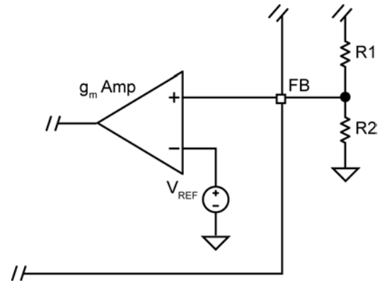
Figure 7. Voltage-Divider Configuration
