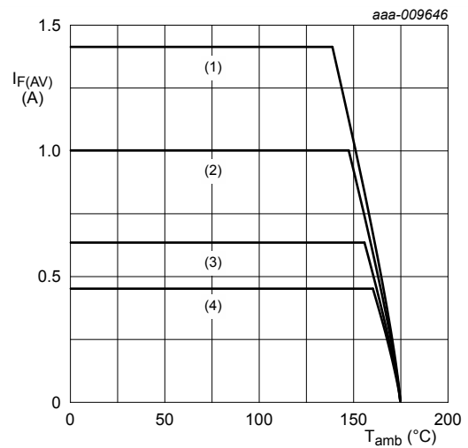
Ceramic PCB, \text{Al}_2\text{O}_3 , standard footprint T_j = 175\text{ °C} (1) \delta = 1 (DC) (2) \delta = 0.5; f = 20\text{ kHz} (3) \delta = 0.2; f = 20\text{ kHz} (4) \delta = 0.1; f = 20\text{ kHz}
